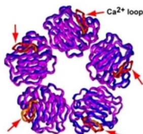
Figure 1. Structure of C-Reactive Protein
