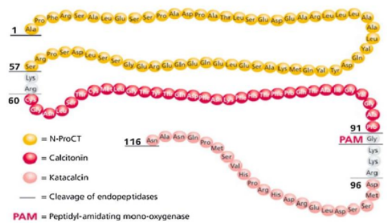
Figure 3. Structure of Procalcitonin
